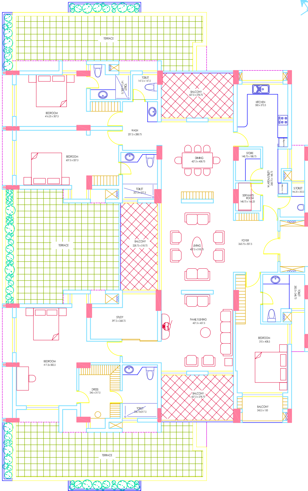
5 12th FLOOR PLAN ( 12 C ) SCALE : 1 : 50
